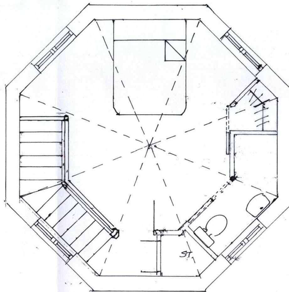
FIRST FLOOR 1:50
