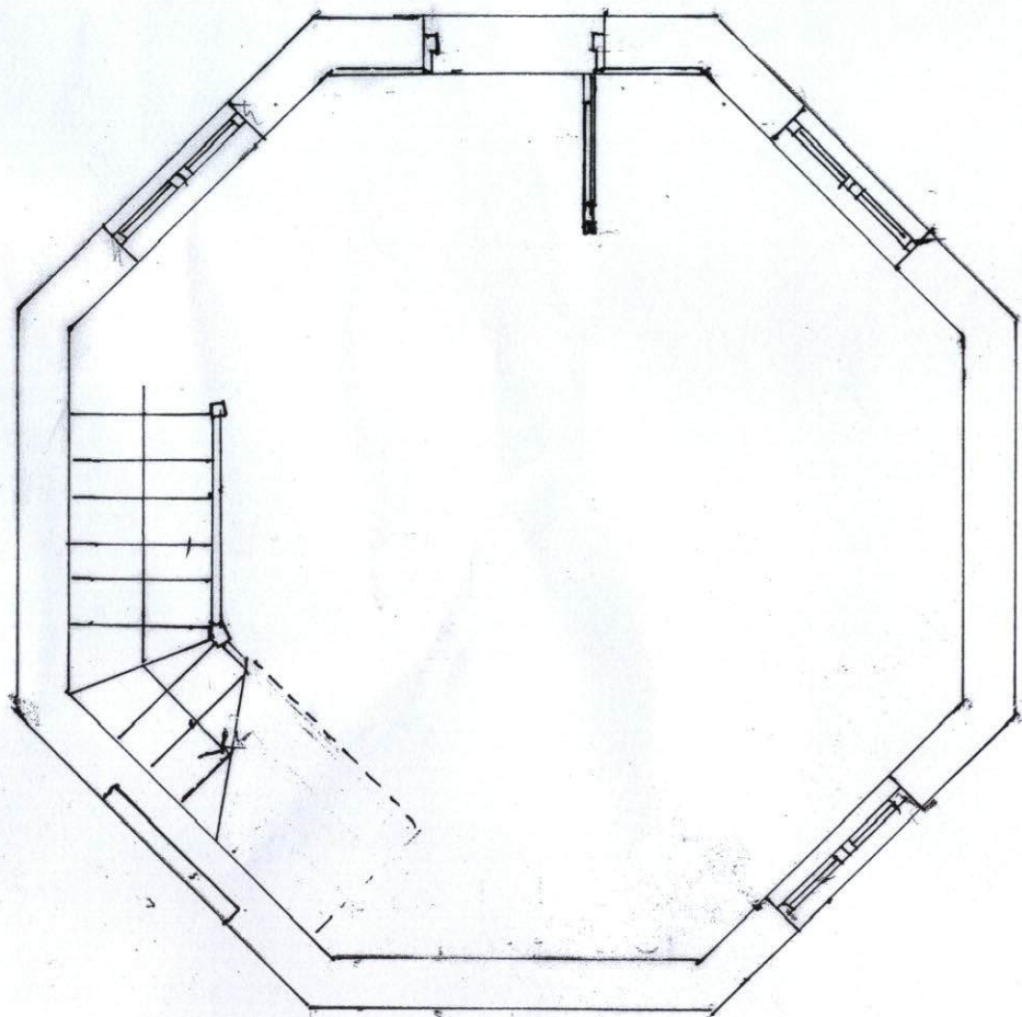
GROUND FLOOR 1:50
